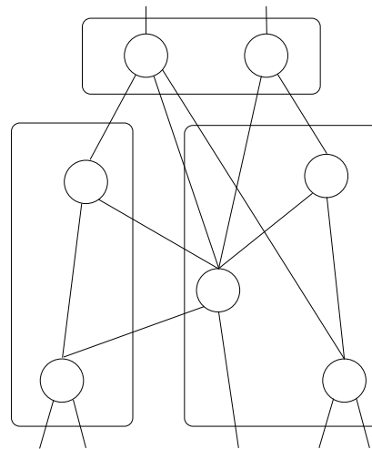
Figure 1. Multi-level circuit clustered into a network of PLAs.
