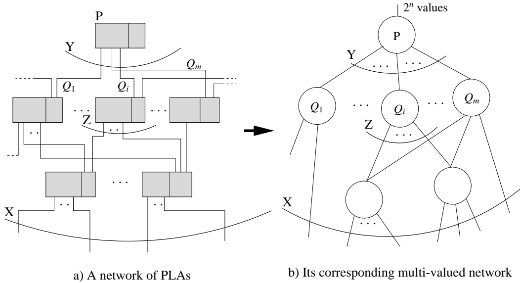
Figure 3. Multi-valued SPFD based wire removal.
